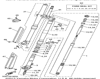
Front fork
