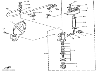
Rear master cylinder
