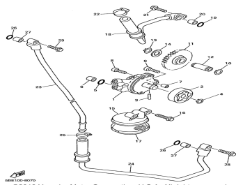
Oil pump
