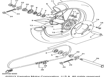
Rear wheel
