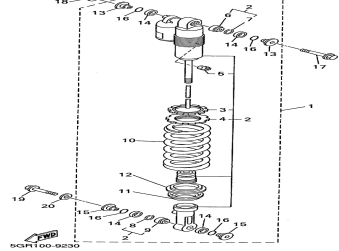
Rear suspension
