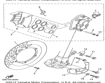
Front brake caliper
