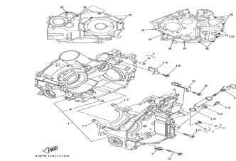
©2014 Yamaha Motor Corporation, U.S.A. All rights reserved. Картер двигателя
