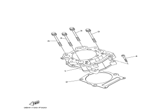
©2014 Yamaha Motor Corporation, U.S.A. All rights reserved. Цилиндр
