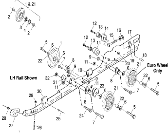
Rail mounting (suspension) - s01st5bs
