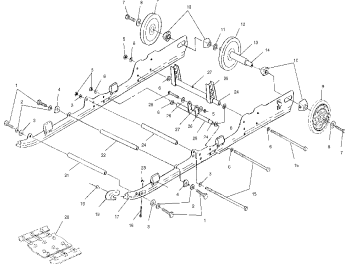
Suspension - s01st5bs
