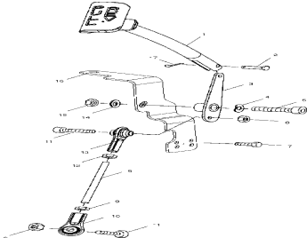
Reverse linkage - s01st5bs
