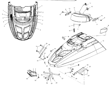
Hood - s01st5bs
