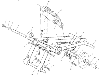
Front torque arm - s01st5bs
