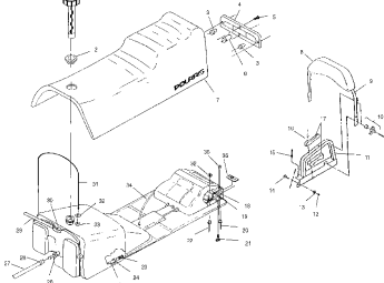
Seat and gas tank - s01st5bs
