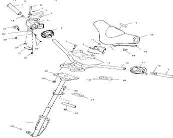
Steering - handlebar - s01st5bs
