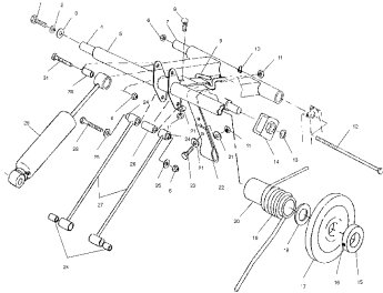
Rear torque arm - s01st5bs
