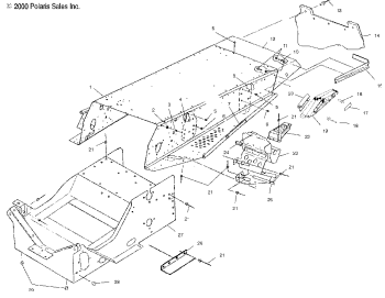
Tunnel - s01st5bs
