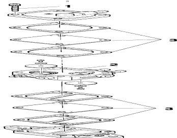
Fuel pump - s01sd5bs
