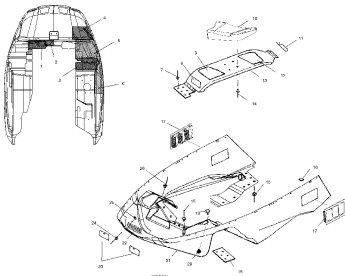
Nosepan - s01st5bs
