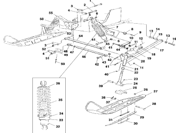
Front suspension and ski - s01st5bs
