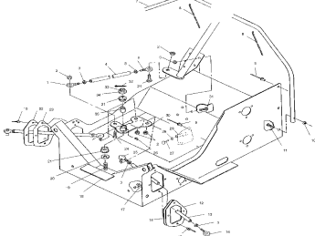
Steering - s01st5bs
