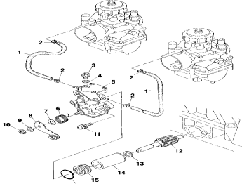
Oil pump - s01sd5bs
