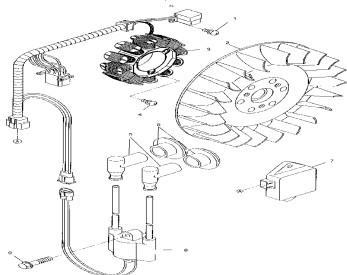
Magneto - s01sr5bs
