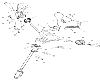
Steering - handlebar - s01sr5bs
