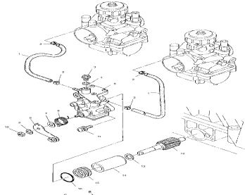
Oil pump - s01sr5bs
