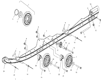
Rail mounting suspension - s01sr5bs
