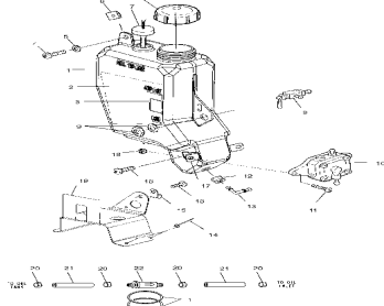
Oil tank - s01sr5bs
