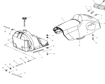
Seat and gas tank - s01sr5bs
