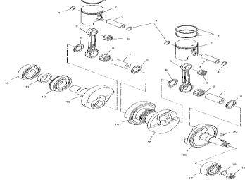
Piston and crankshaft - s01sr5bs
