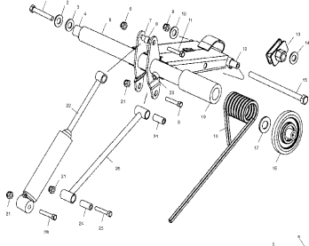
Rear torque arm - s01sr5bs
