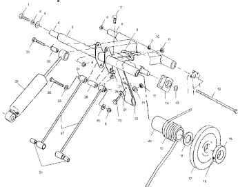
Rear torque arm - e99ss6du
