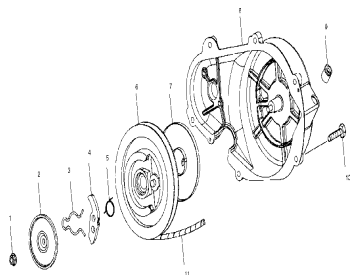
Recoil starter - e99ss6du
