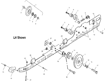
Rail mounting (suspension) - e99ss6du
