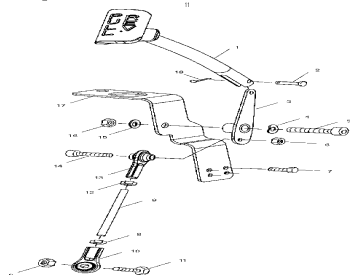
Reverse linkage - e99ss6du
