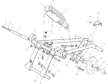
Front torque arm - e99ss6du
