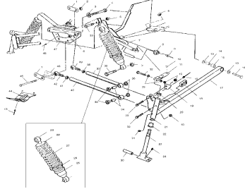
Front suspension - e99ss6du
