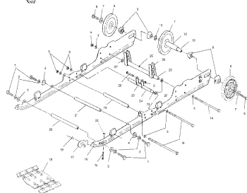
Suspension - e99ss6du
