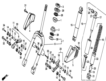
Front fork
