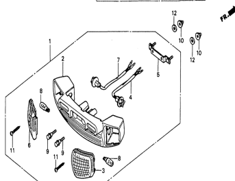
Rear turn signal
