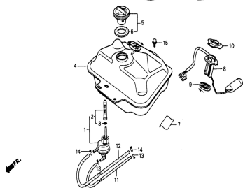
Fuel tank
