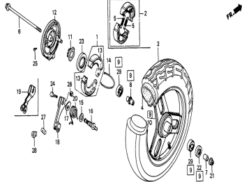
Front wheel
