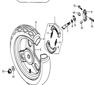
Rear wheel
