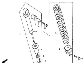
Rear shock absorber
