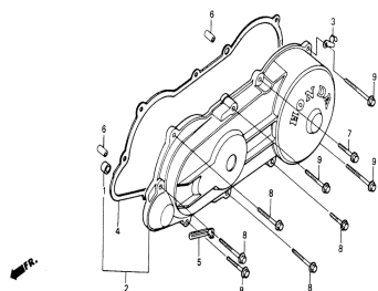
Left side cover 88-93
