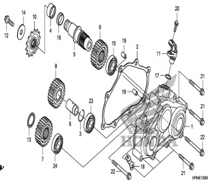
Reduction gear
