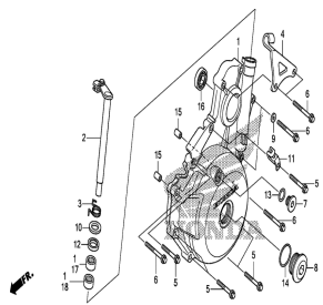
Left crankcase cover
