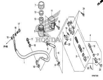
Rear brake mastercylinder
