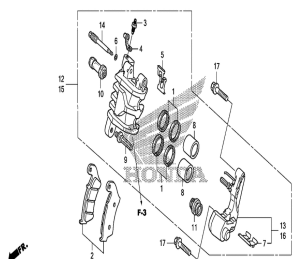
1P961200 Front brake caliper
