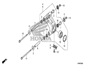
Rear knuckle
