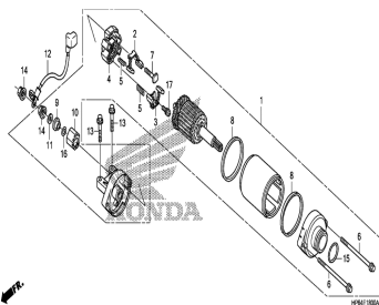
Starter motor
