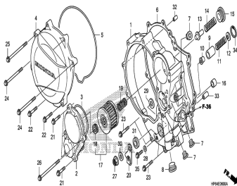
Right crankcase cover
