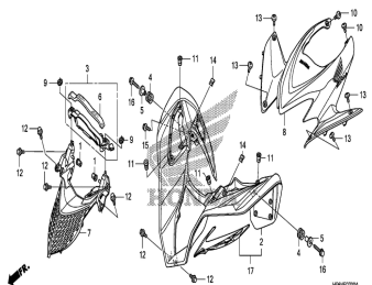
Front fender
