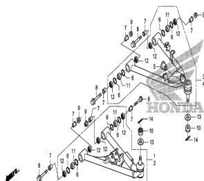
1P961000 Front arm
