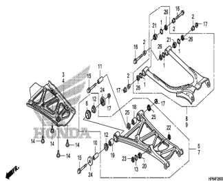
Rear arm
