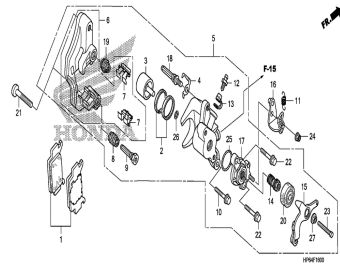
Rear brake caliper
