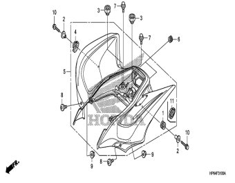
Rear fender
