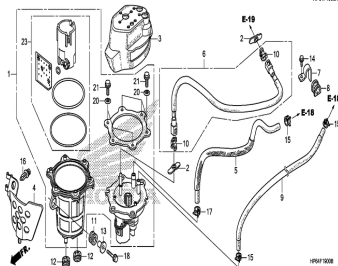
Fuel pump
