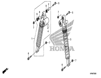
Rear shock absorber
