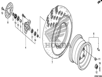
Front wheel
