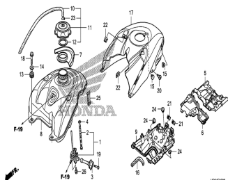
Fuel tank
