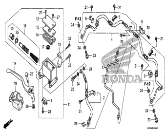
Front brake mastercylinder
