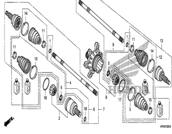
Rear driveshaft
