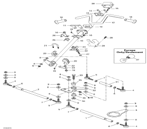
Steering system
