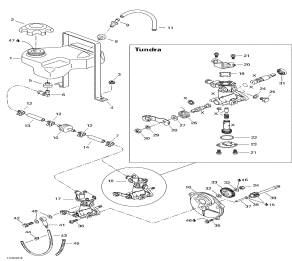
Oil injection system
