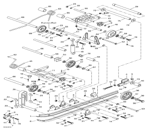
Rear suspension
