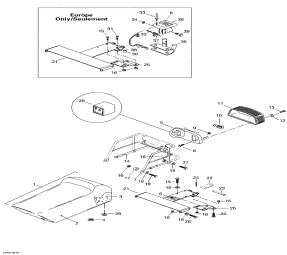
Frame and body
