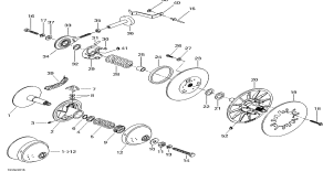
Pulleys
