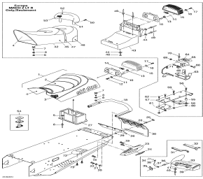
Seat and accessories
