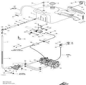
Fuel system
