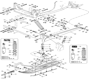
Front suspension and ski
