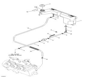
Oil tank
