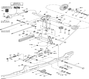
Rear arm, rear suspension
