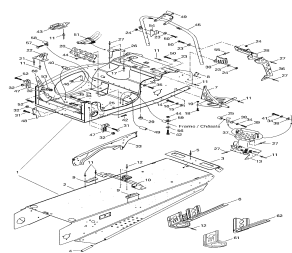
Frame and accessories
