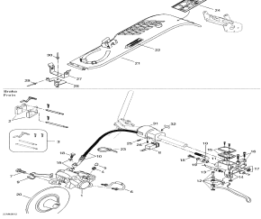
Hydraulic brake and belt guard
