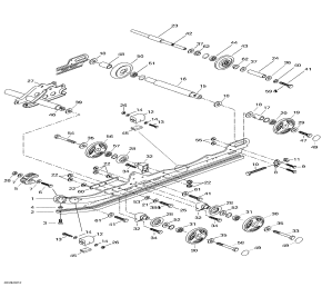
Rear suspension
