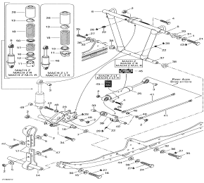
Front arm, rear suspension
