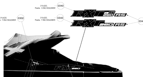
DETAIL ITEM 0302, 0340, 0345.
