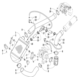
Intercooler assembly
