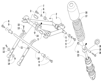
Rear suspension front arm assembly
