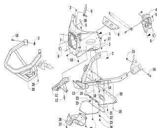
Front bumper and frame assembly
