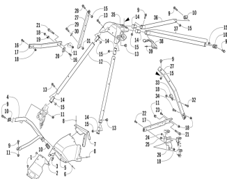
Steering support assembly
