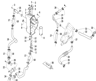
Oil tank assembly
