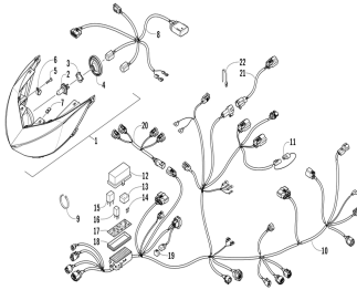
Headlight and wiring assemblies
