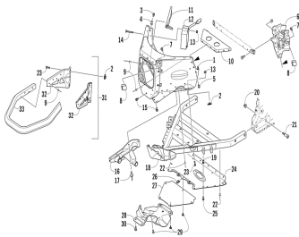
Front bumper and frame assembly
