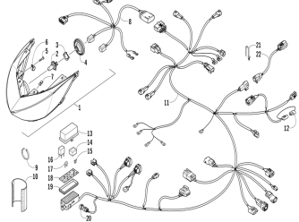
Headlight and wiring assemblies
