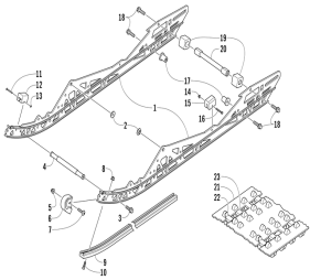
Slide rail and track assembly
