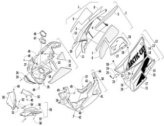
Skid plate and side panel assembly
