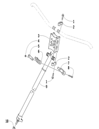
Steering post assembly
