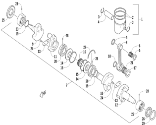
Piston and crankshaft
