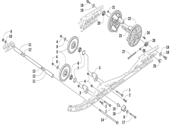
Idler wheel assembly
