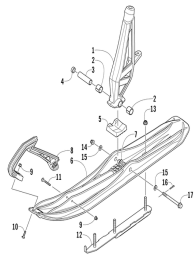
Ski and spindle assembly
