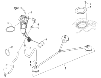
Fuel pump assembly
