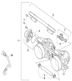
Throttle body assembly
