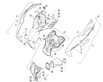
Hood and air intake assembly
