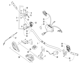
Handlebar and controls
