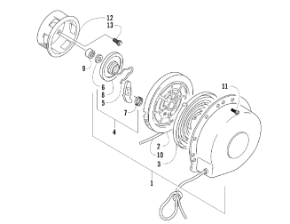
Recoil starter
