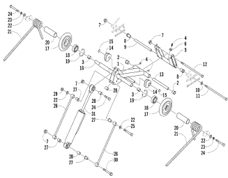
Rear suspension rear arm assembly
