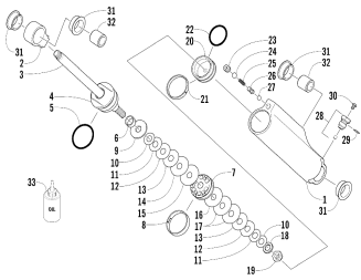
Rear suspension rear arm shock absorber (ext_int)
