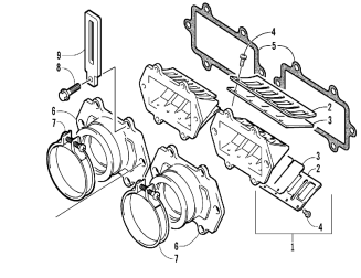
Reed valve assembly
