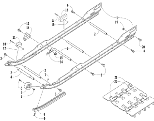
Slide rail and track assembly (ext_international)
