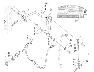
Reverse shift lever assembly (lx_ext_international)
