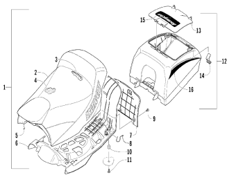
Seat and storage box assembly
