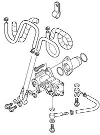
Oil pump
