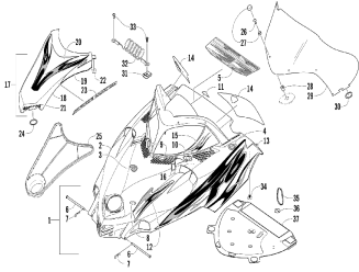
Hood and windshield assembly
