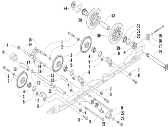
Idler wheel assembly
