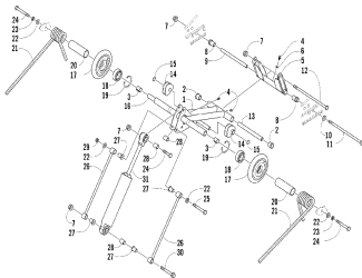
Rear suspension rear arm assembly
