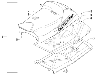
Seat assembly
