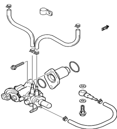
Oil pump
