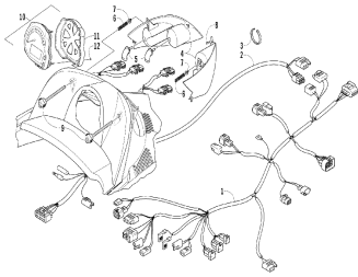
Headlight instruments and wiring assemblies
