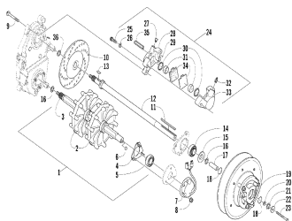
Drive train shafts and brake assemblies
