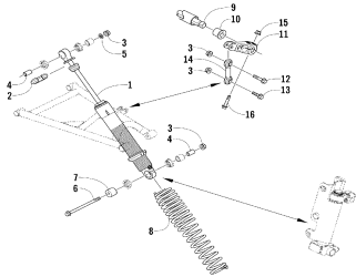
Shock absorber and sway bar assembly
