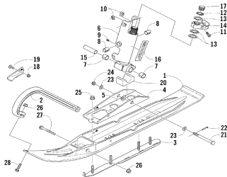
Ski and spindle assembly
