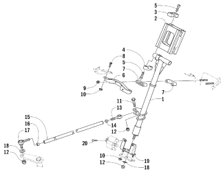
Steering post assembly
