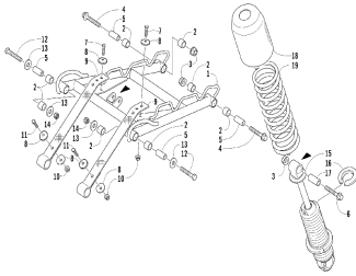
Rear suspension front arm assembly
